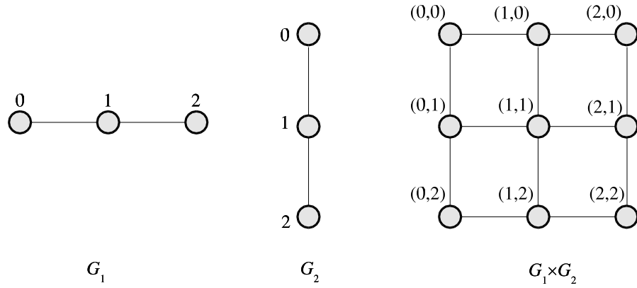
Figure 1: A homogeneous two-dimensional mesh
