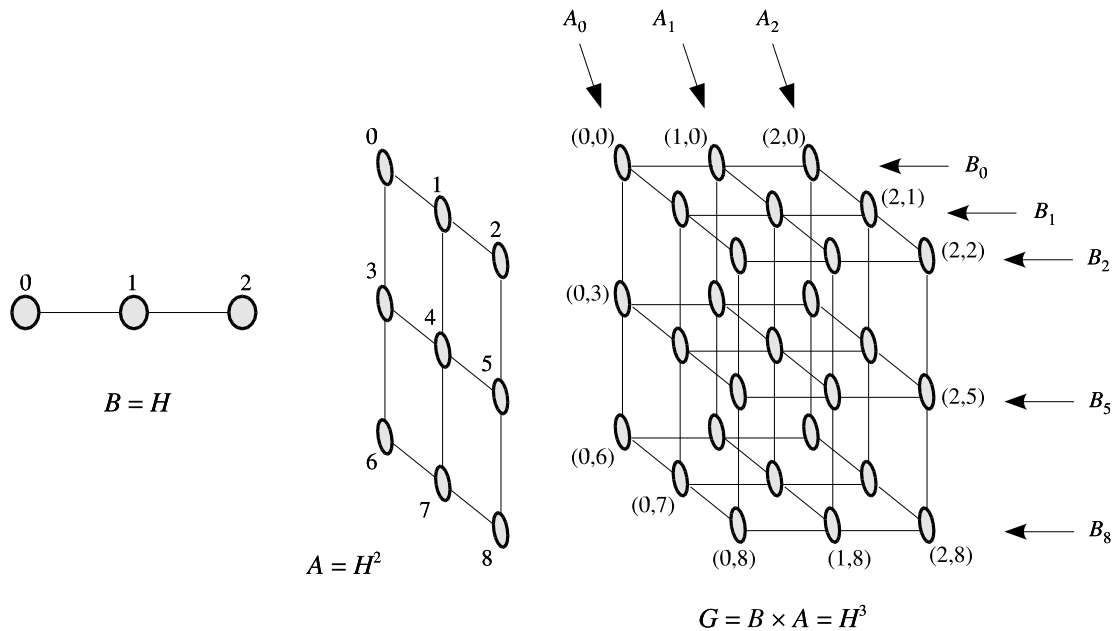
Figure 2: A homogeneous three-dimensional mesh
