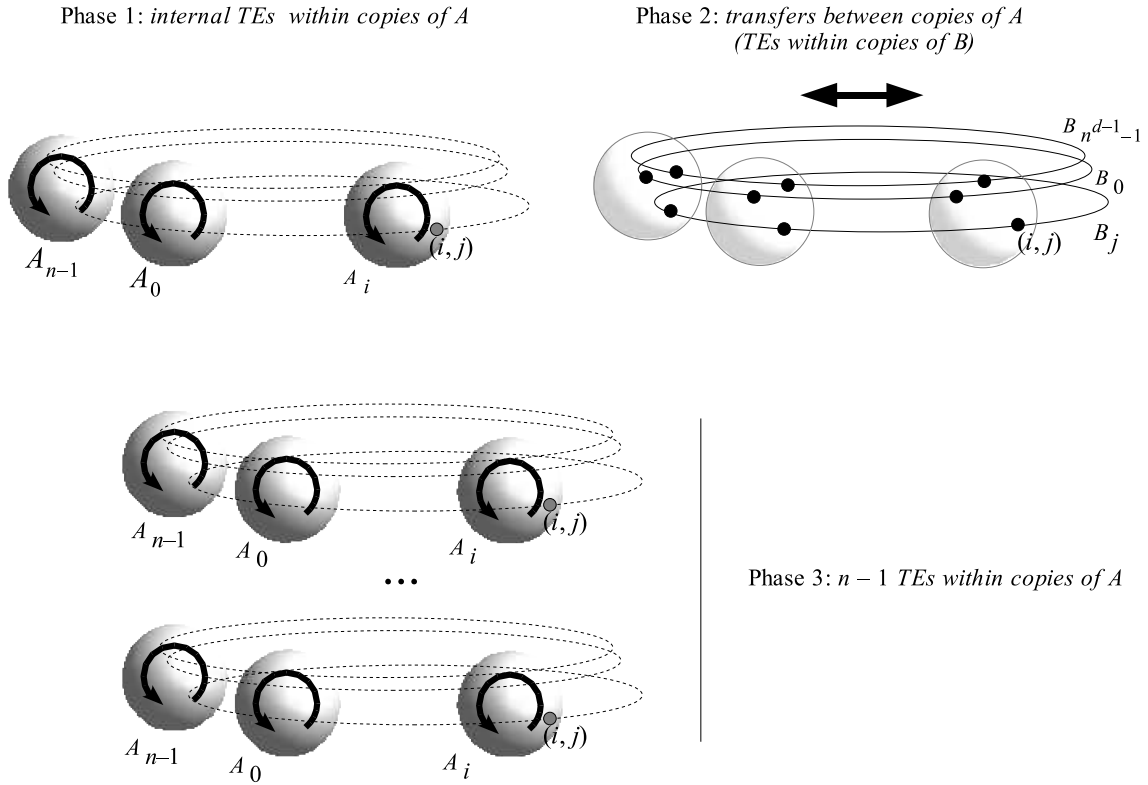
Figure 4: Total exchange in a general multidimensional network
